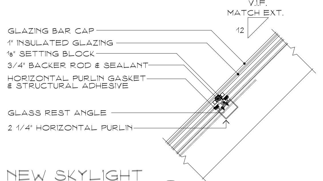
NEW SKYLIGHT PURLIN DETAIL SCALE: 1 1/2" = 1'-0"
