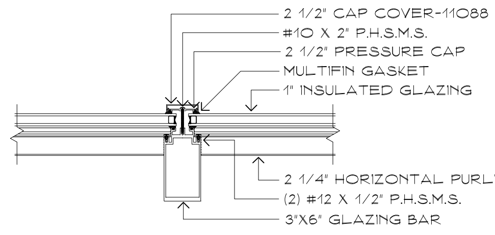
NEW SKYLIGHT RAFTER DETAIL SCALE: 1 1/2" = 1'-0"
