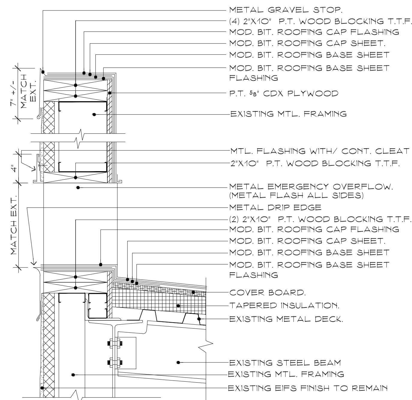
E.M. OVERFLOW DETAIL SCALE: 1/2" = 1'-0"
