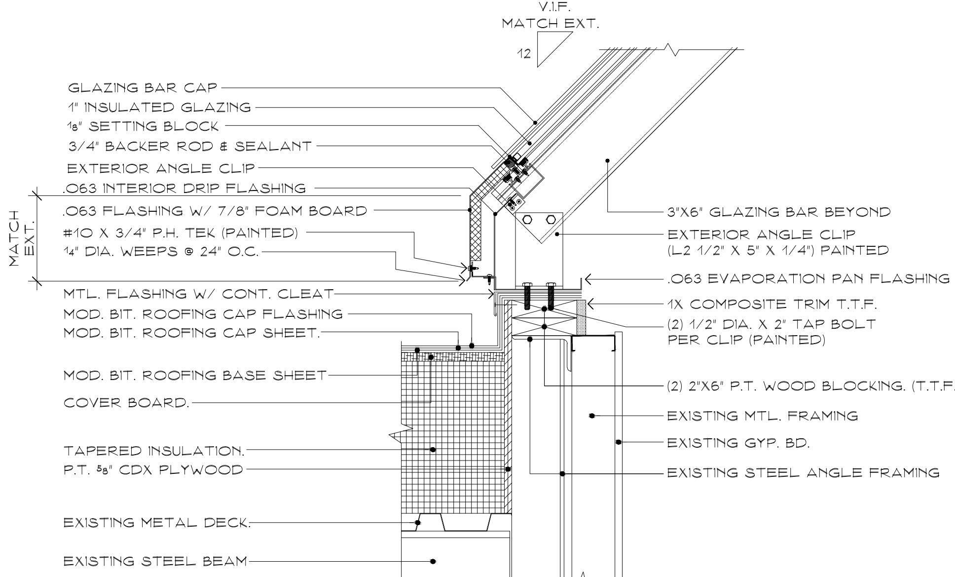
SKY LIGHT DETAIL SCALE: 1/2" = 1'-0"
